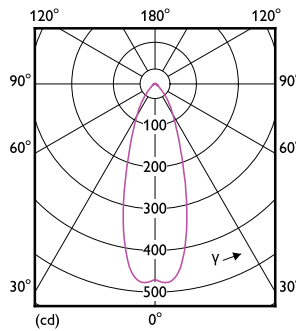
LEDspots Corepro SLR 3W PAR16 GU10 840 36D-LDD
