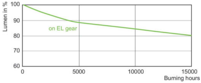
Lumen Maintenance Diagram - MASTER CDM-TC Elite 50W/930 G8.5 1CT/12
