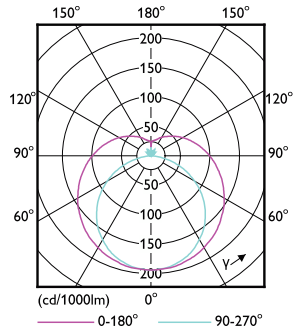
Light Distribution Diagram - CorePro LEDtube HF 1500mm HO 26.7W 840T5
