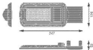
URBAN LITE M 50W
