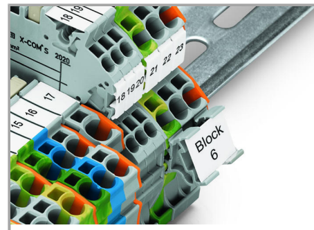
Marker carrier (2009-198)
