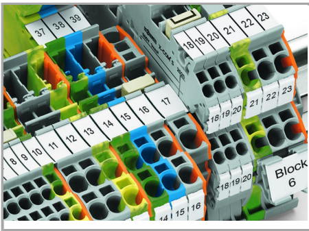
Commoning X-COM ® S-SYSTEM Terminal Blocks using jumpers for TOPJOB ® S Terminal Blocks. An end plate provides connection to TOPJOB ® S Terminal Blocks. 2020 and 2022 Series Terminal Blocks are combinable. Jumper slots are on the same level for both series.
