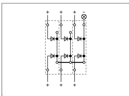
Collective fault signals can be created using the following terminal blocks:
